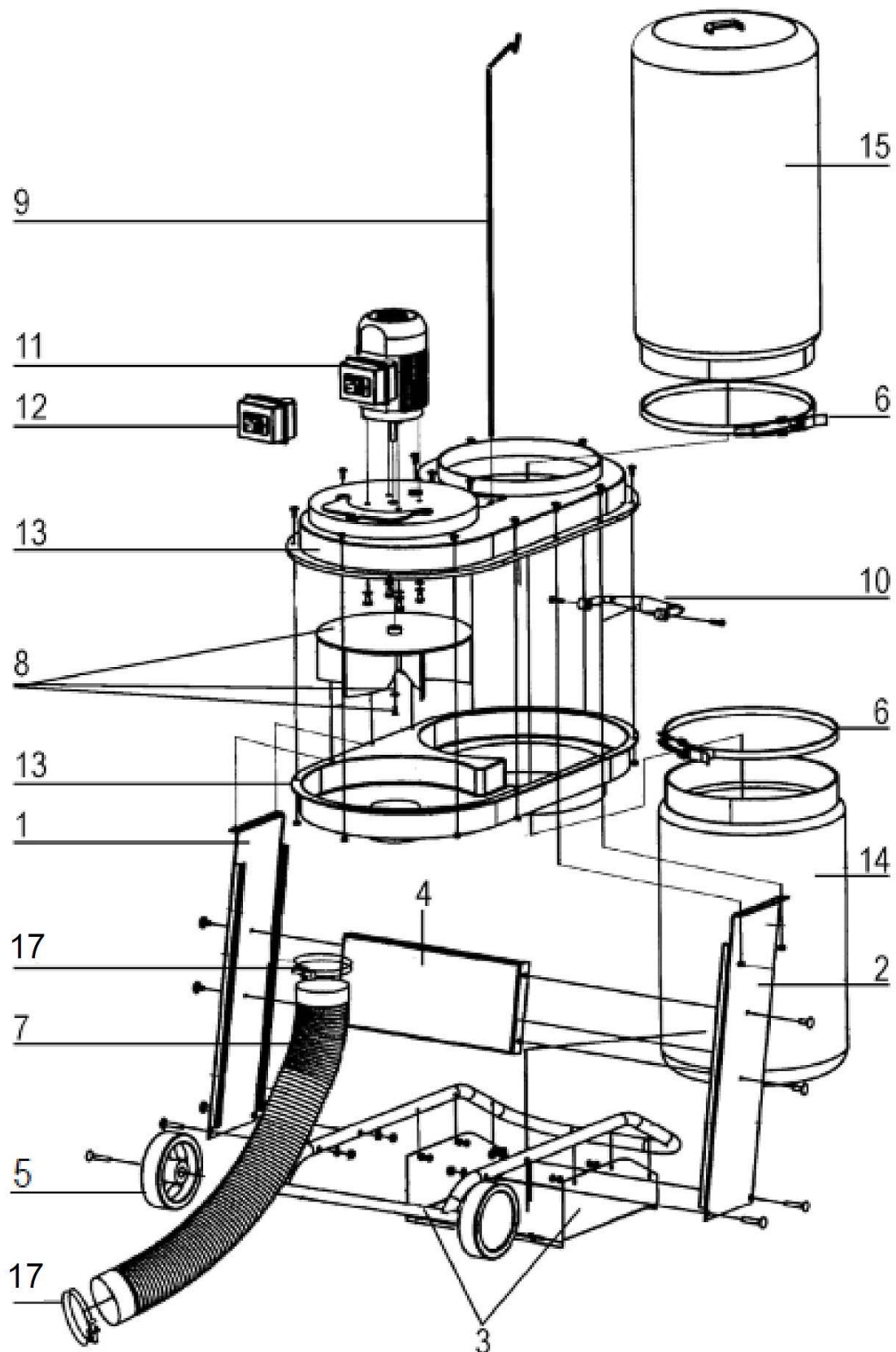
Fig. 14: Spare parts drawing SAA 902
