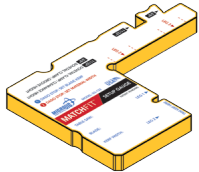
Setup Gauge SG-133
